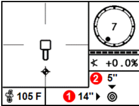
Locate screen with Target Steering Mode on
